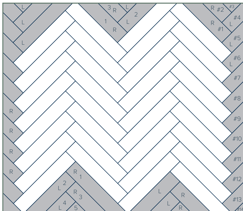
FIGURE 6 : Completing cut sections of the floor
